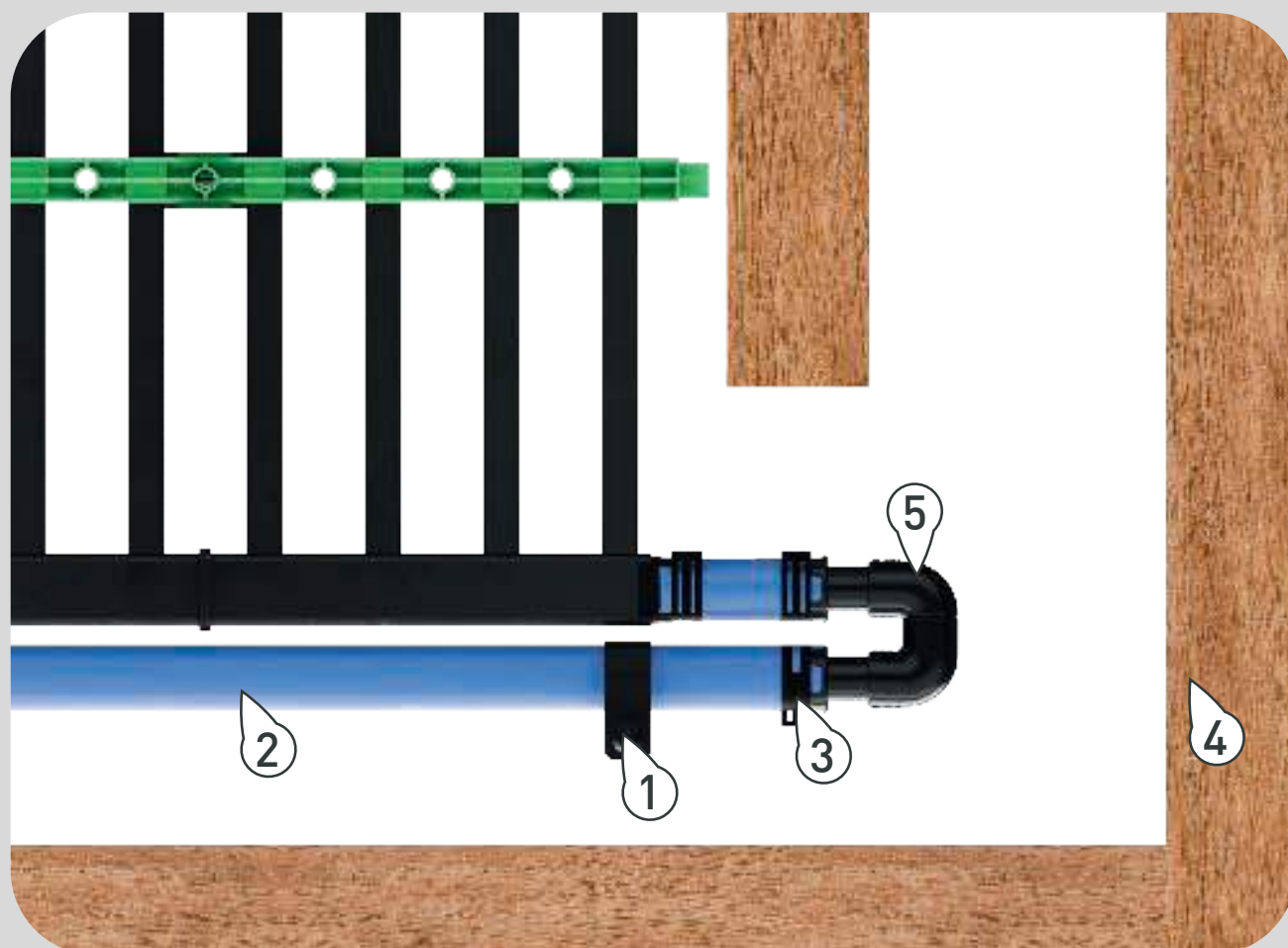
Detail: Connection
