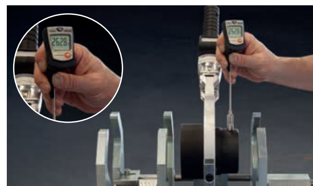
Temperature measurement on aquatherm welding machine
