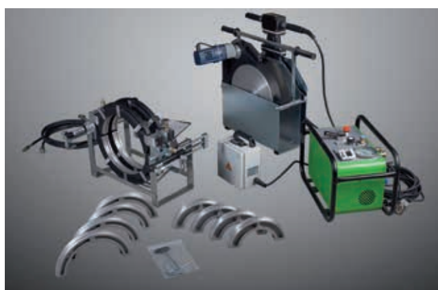
Butt fusion machine type Light including accessories
